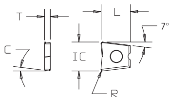
ZCEA / G Insert Dimensional and Grade Specifications
