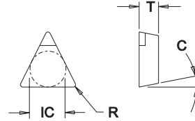
PCD / CBN Insert Dimensional & Grade Specifications
