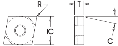
PCD / CBN Insert Dimensional & Grade Specifications
