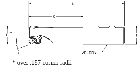
Extended Reach • 7° Backdraft Configuration
