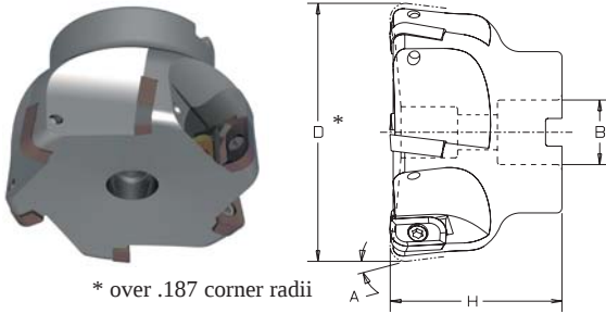
7° Backdraft • Ramping Capability Configuration
